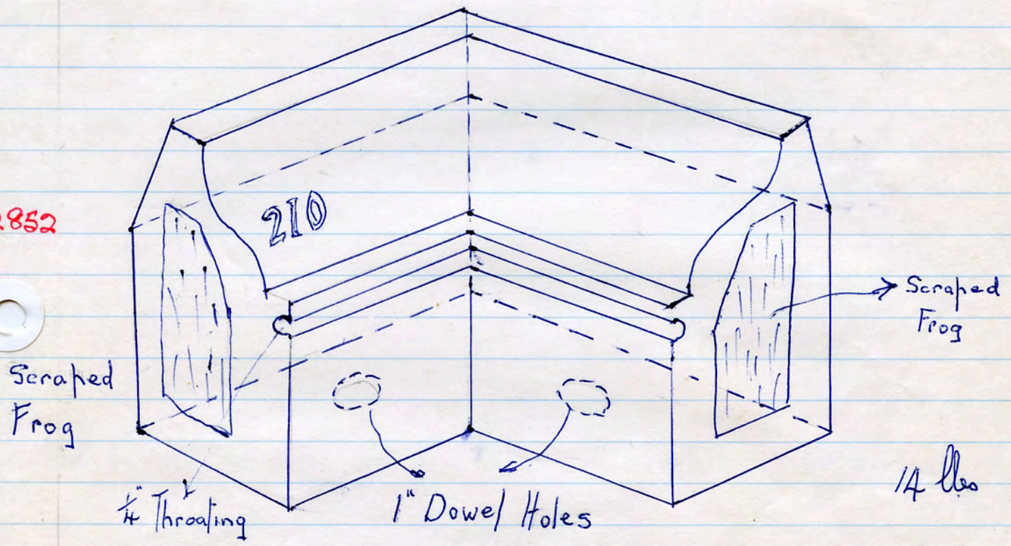
red T.C. return mould (aprow) for window.
